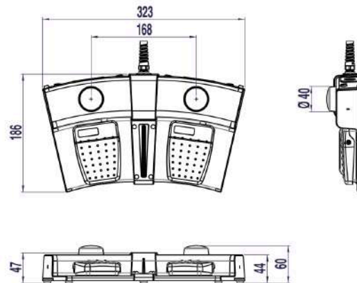
Modular base
