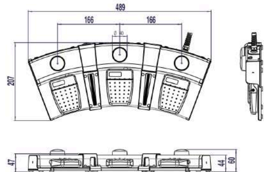
Modular base
