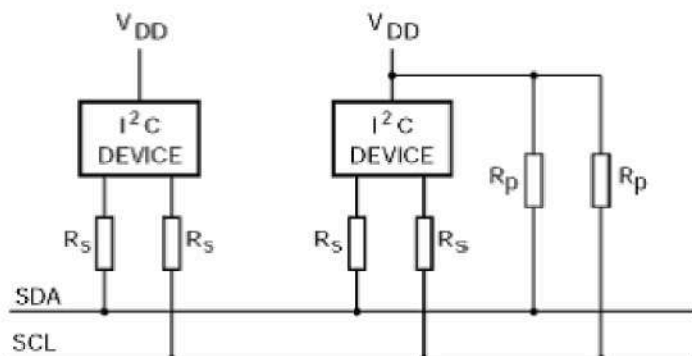
Figure 4: I2C-bus with a protection resistor R_S in the leads of the bus devices
