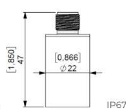
M12x1 (S763)
