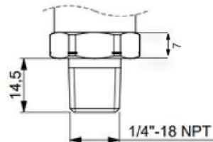
Option "H"
