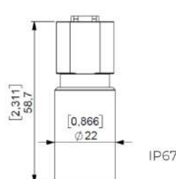
DT04-4P
