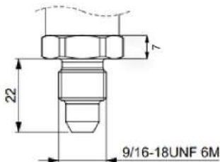
Option "E"
