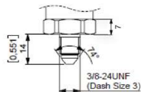
Option "H"
