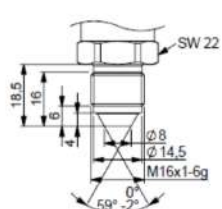
Option "M16"
