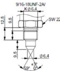
Option "O"
