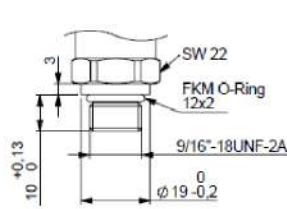
Option "P"
