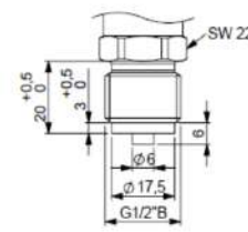
Option "G1/2B"
